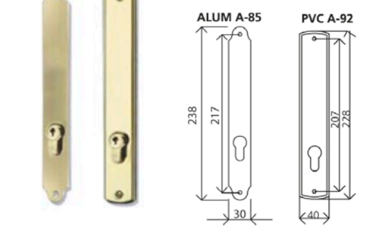
REF. 10 REF. 20 LONG KEYHOLE
