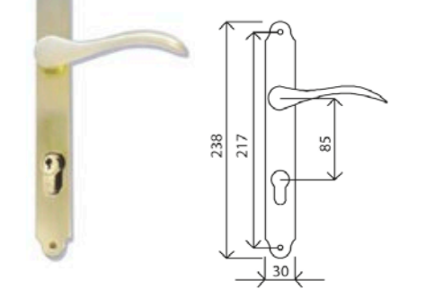
REF. 11 ALUMINIUM HANDLE SET A-85
