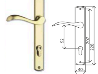
REF. 21 HANDLE PVC A-92
